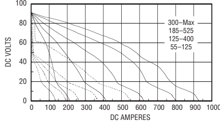
VOLT/AMP CURVE – STICK MODE
